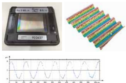
Specimen rugozitate 3 \mu\text{m}
